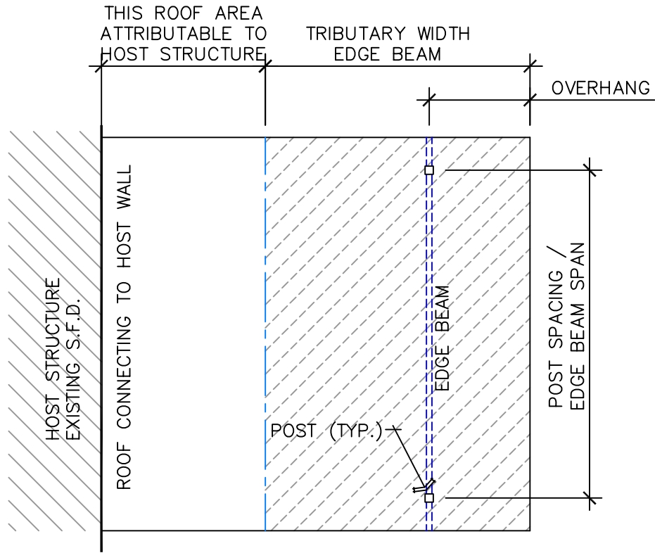
SCHEMATIC PARTIAL PLAN / TRIBUTARY LOAD WIDTHS
