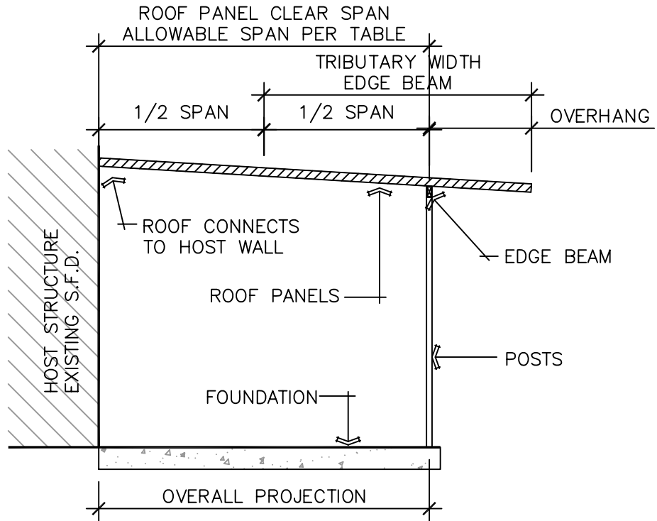
SCHEMATIC SECTION / TRIBUTARY LOAD WIDTHS
