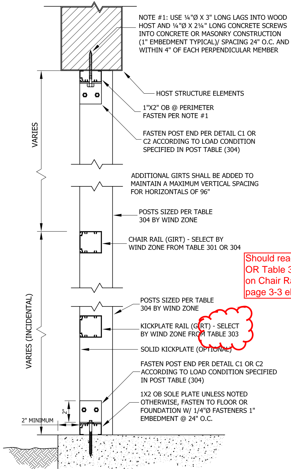
TYPICAL SECTION / SCREEN WALL WITHOUT GUARDRAIL (NOT SUPPORTING ROOF)
