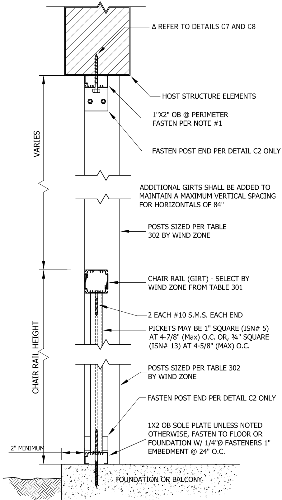
TYPICAL SECTION / SCREEN WALL W/GUARDRAIL CHAIR RAIL HEIGHT @ 42" (COMMERCIAL) OR 36" (RESIDENTIAL)
