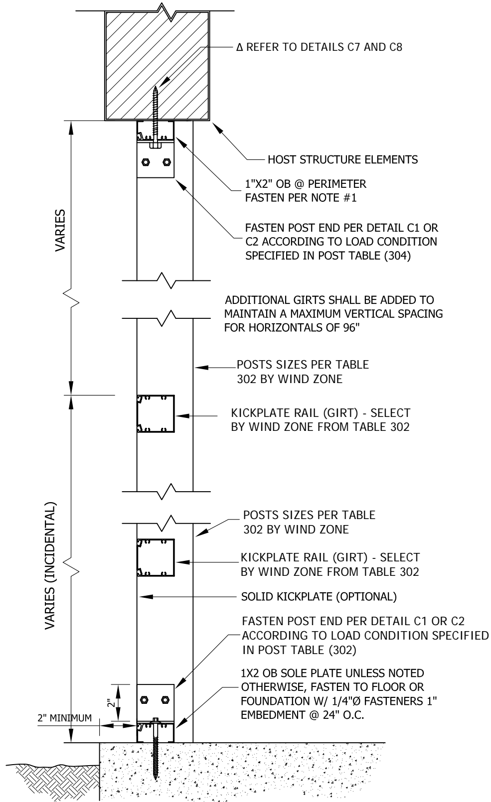
TYPICAL SECTION / SCREEN WALL WITHOUT GUARDRAIL (NOT SUPPORTING ROOF) FOUNDATION OR BALCONY
