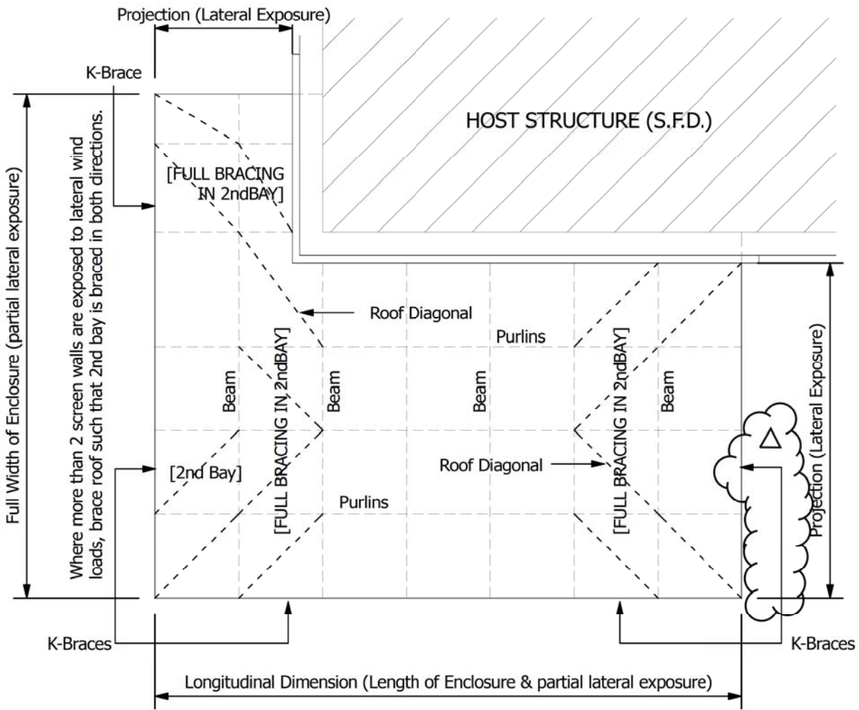
Screen Enclosure Roof Bracing Strategies - Schematic #4
