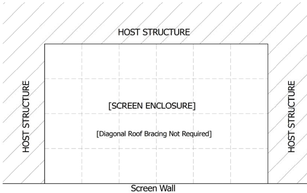
Screen Enclosure Roof Bracing Strategies - Schematic #1
