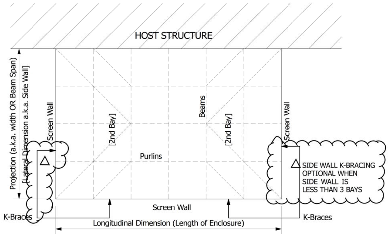
Screen Enclosure Roof Bracing Strategies - Schematic #2
